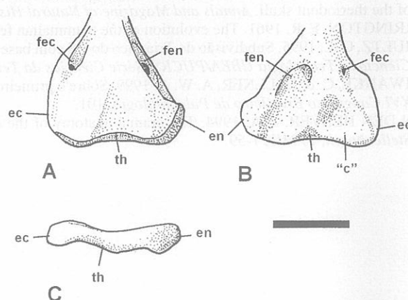
Figure 7. A, dorsal; B, ventral and C, distal views of the distal portion of the right humerus of Thrinaxodon . Abbreviations: "c", capitulum; ec, ectepicondyle; en, entepicondyle; fec, ectepicondylar foramen; fen, entepicondylar foramen; th, trochlea (modified from Jenkins, 1971). Scale 1 cm.
