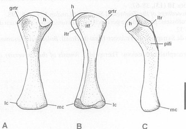
Figure 6. A, dorsal; B, ventral and C, medial views of the femur of Thrinaxodon . Abbreviations: grtr, greater trochanter; h, head; itf, intertrochanteric fossa; lc, lateral condyle; ltr, lesser trochanter; mc, medial condyle; pifi, puboischiofemoralis internus muscle insertion (modified from Jenkins, 1971). Scale 1 cm.
