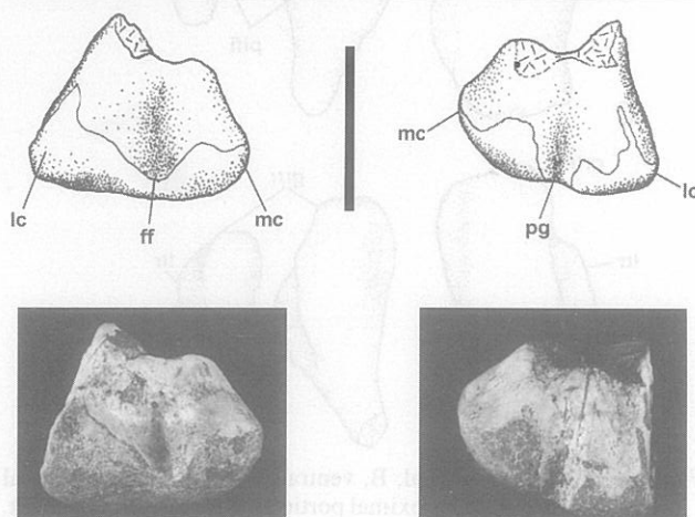
Figure 4. Ventral and dorsal view of the distal portion of femur (UFRGS PV 353 T). Abbreviations: ff, flexor fossa; lc, lateral condyle; mc, medial condyle; pg, patellar groove. Scale 1 cm.
