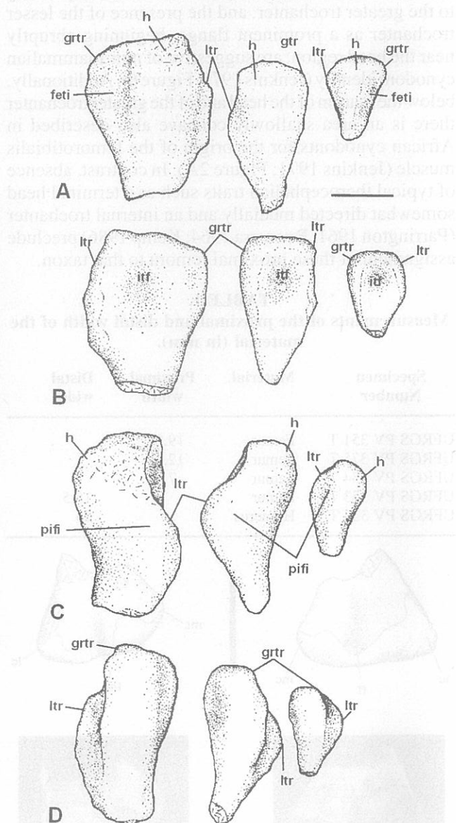
Figure 3. A, dorso-medial; B, ventral; C, medial and D, lateral views of the proximal portions of femora. Left to right, UFRGS PV 351 T; UFRGS PV 375 T and UFRGS PV 354 T. Abbreviations: feti: femorotibialis muscle insertion; grtr, greater trochanter; h, head; itf, intertrochanteric fossa; ltr, lesser trochanter; pifi, puboischiofemoralis internus muscle insertion. Scale 1 cm.
