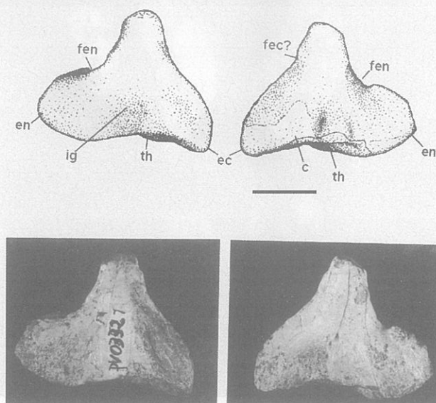
Figure 5. Dorsal and ventral views of the distal portion of humerus (UFRGS PV 332 T). Abbreviations: c, capitulum; ec, ectepicondyle; en, entepicondyle; fec?, ectepicondylar foramen; fen, entepicondylar foramen; ig, intercondylar groove; th, trochlea. Scale 1 cm.
