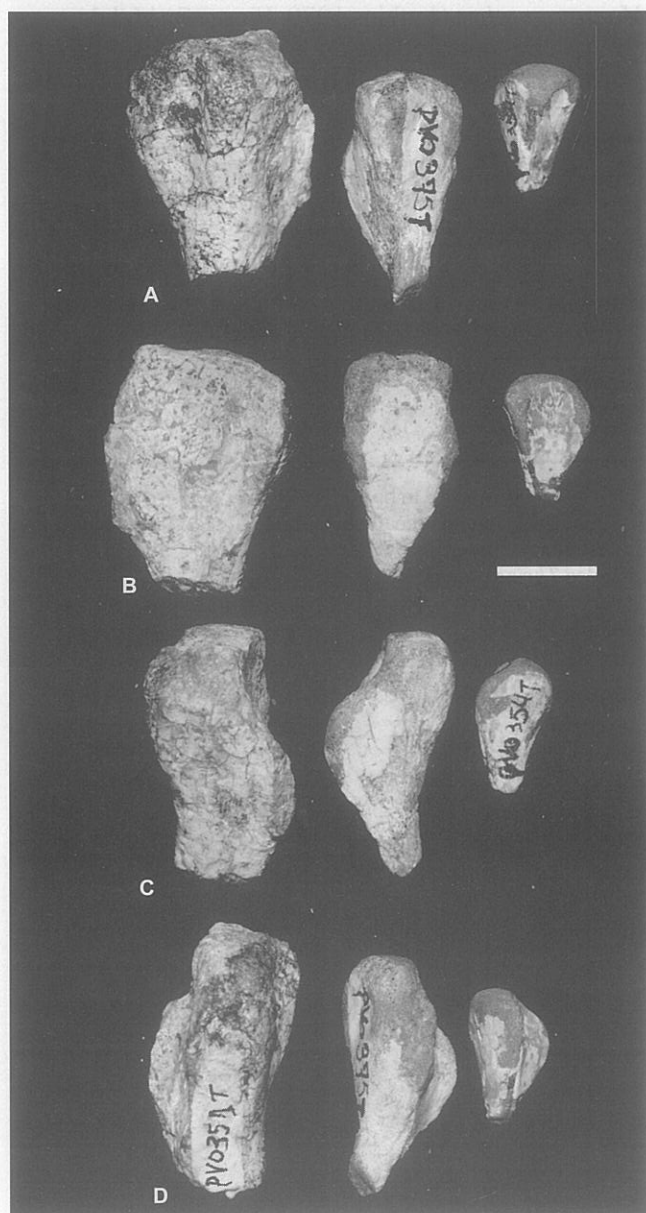
Figure 2. A, dorso-medial; B, ventral; C, medial and D, lateral views of the proximal portions of femora. Left to right, UFRGS PV 351 T; UFRGS PV 375 T and UFRGS PV 354 T. Scale 1 cm.
